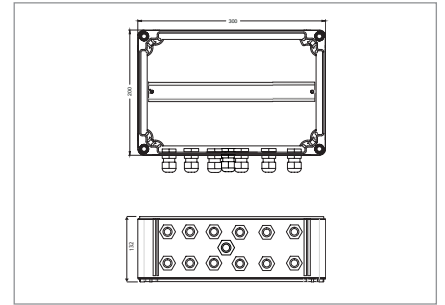
GAK 300 x 200 x 132 mm
