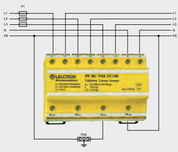
Combined arrester Type 1+2 (V wiring) PowerPro BC at the LPZ transition point O_A - 2^*
