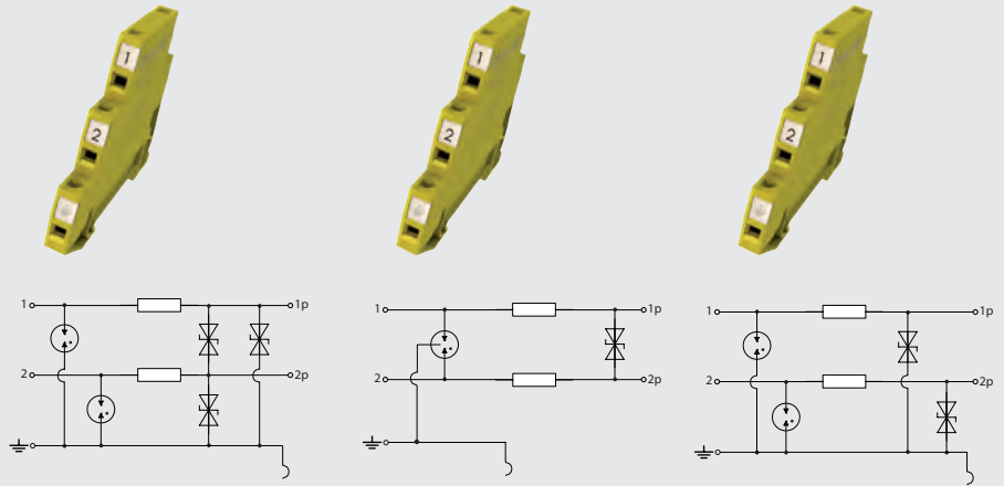
MP RK GDT/Ad-Ad-Pg
