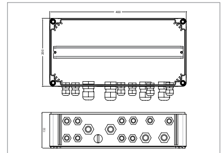
GAK 400 x 200 x 132 mm
