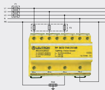
Combined arrester Type 1+2+3 PowerPro BCD at the LPZ transition point O_A - 2^*
